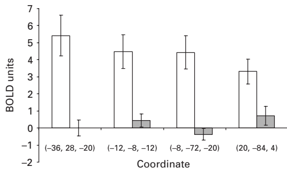
Fig. 3. Areas of significantly increased hemodynamic activity for compulsive hoarding participants ( \square ) versus healthy controls ( \blacksquare ) while deciding whether to discard Participant's Possessions (PP) versus Experimenter's Possessions (EP). Image is thresholded at p < 0.01 .
